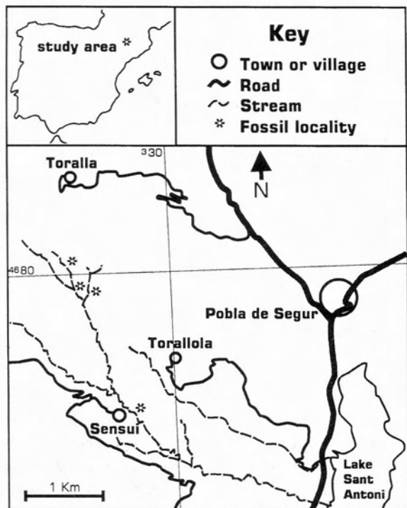
Fig. 1. The fossil localities around Torallola in the Tremp Basin of the Spanish Pyrenees
